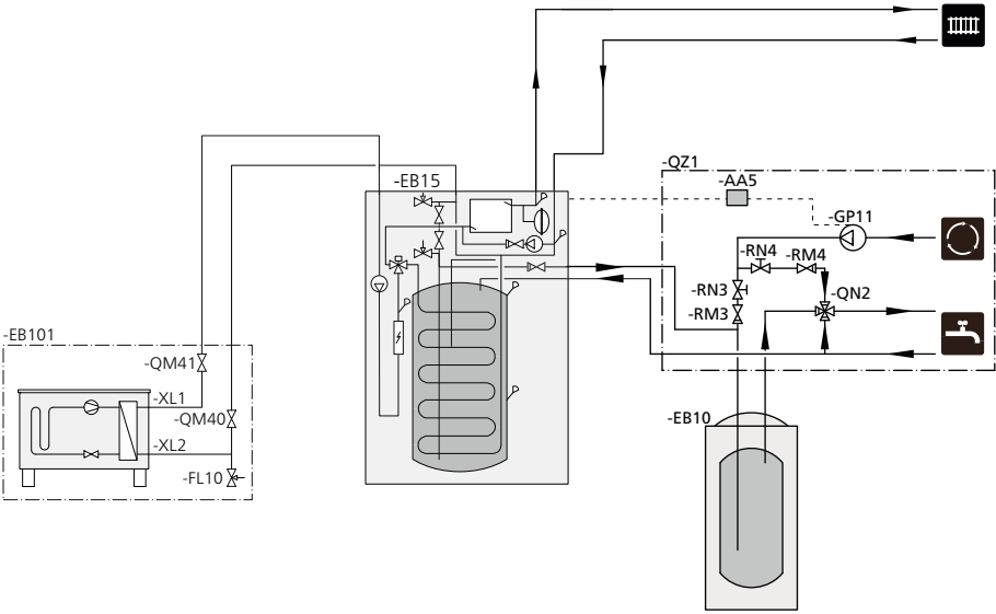
Outline diagram VVM320 with AXC 40 and hot water circulation
