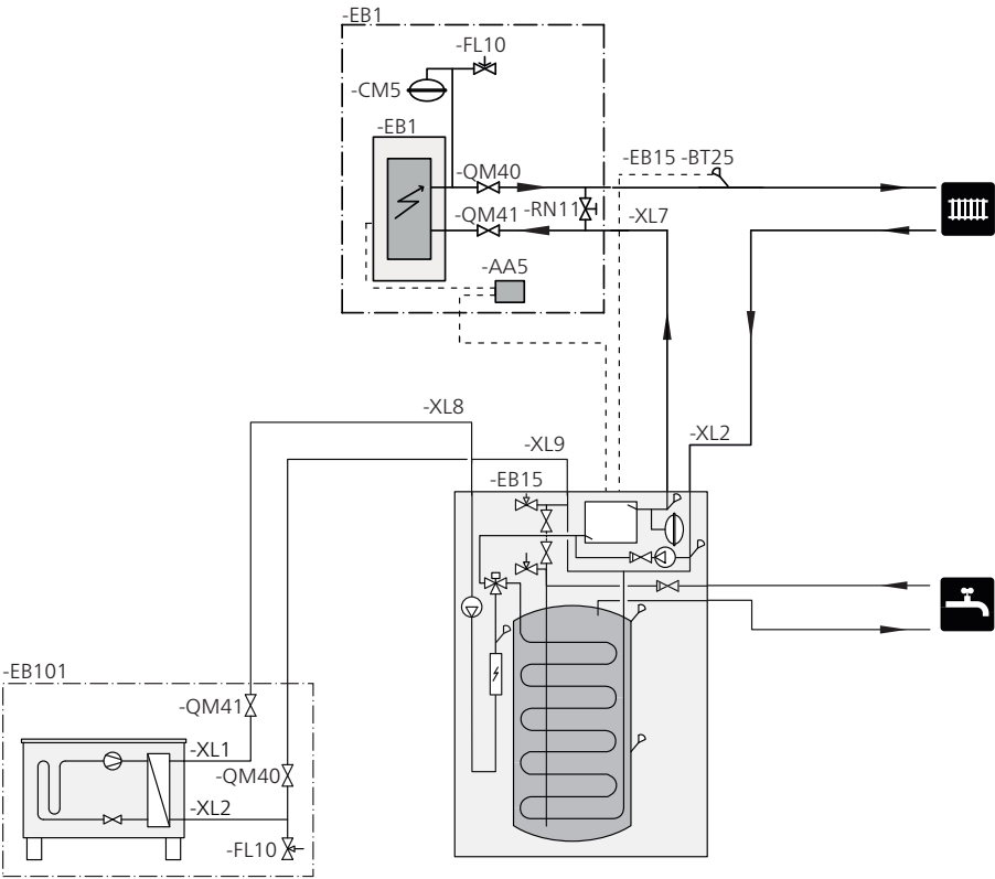
Outline diagram VVM320 with AXC 40 and external addition
