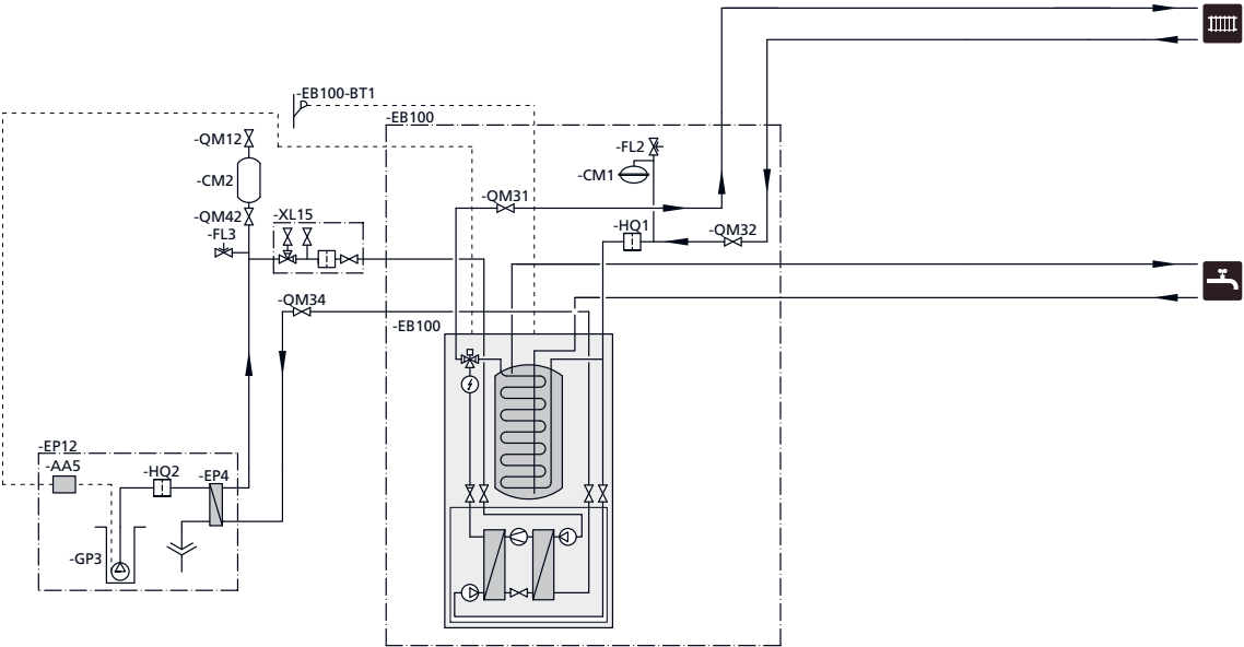
Outline diagram F1245/F1255 with AXC 40 and ground water pump
