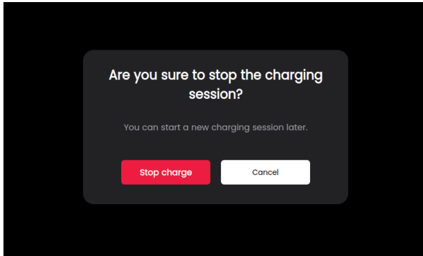
Image 20: confirm stop
